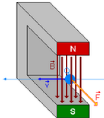
Figure 9: A dipole magnet with a vertical magnetic field and a charged particle moving horizontally through the field. The force is perpendicular to the direction of the magnetic field and the direction of movement of the charged particle, deflecting the charged particle horizontally. Image source: Wikipedia .
