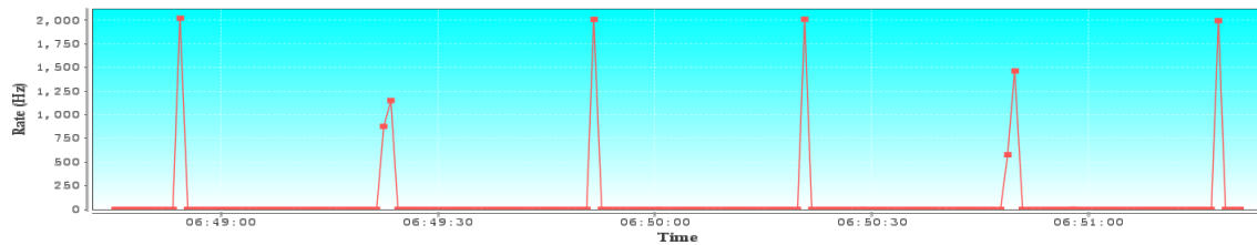
Figure 7: The flux rate at CERN. Particles are not delivered continuously to the experimental area but arrive in spills of approximately. 400 ms duration. Each "spike" in the plot corresponds to one of these spills.
